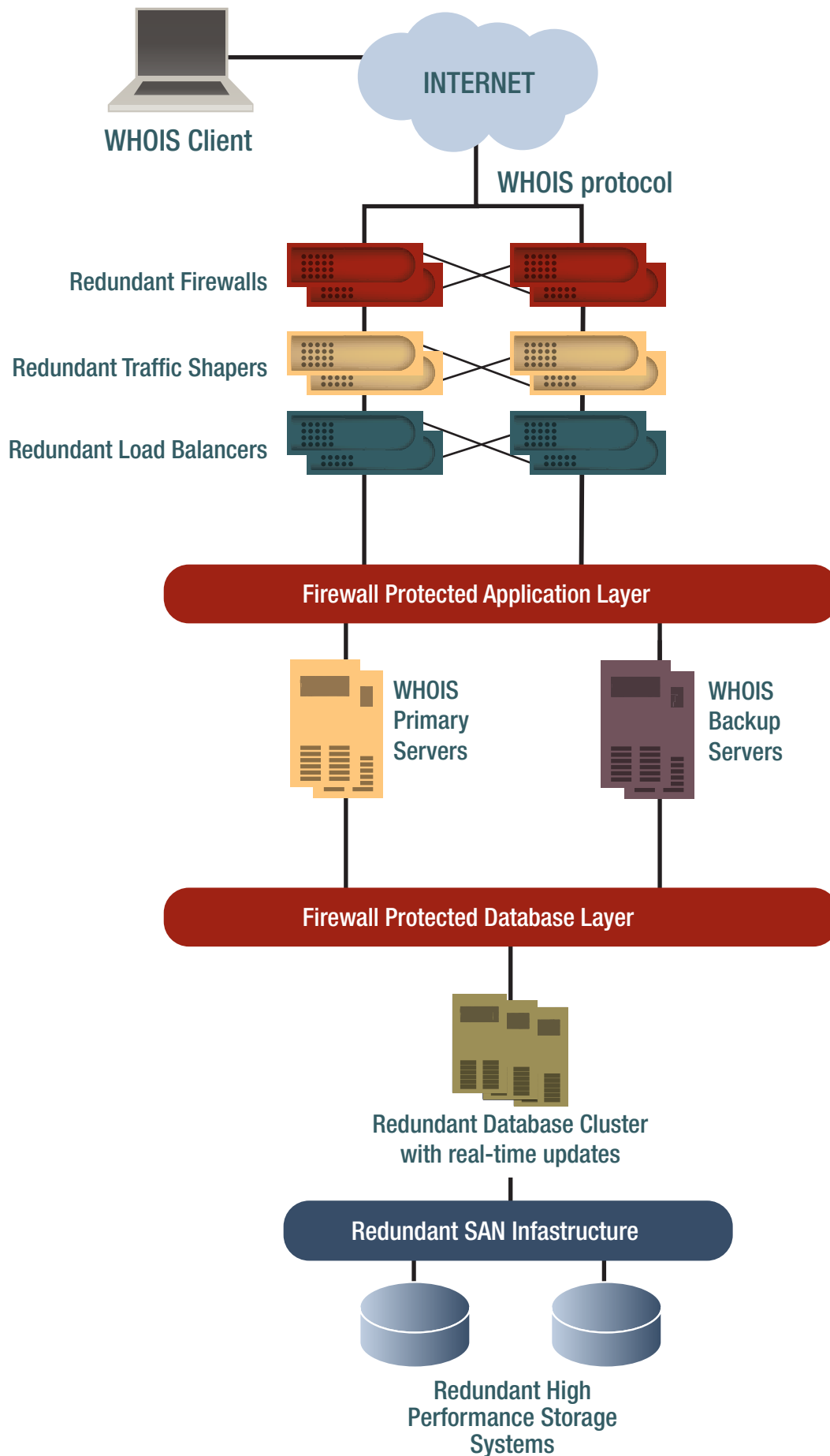
Figure 26-a. Afilias WHOIS service diagram.
