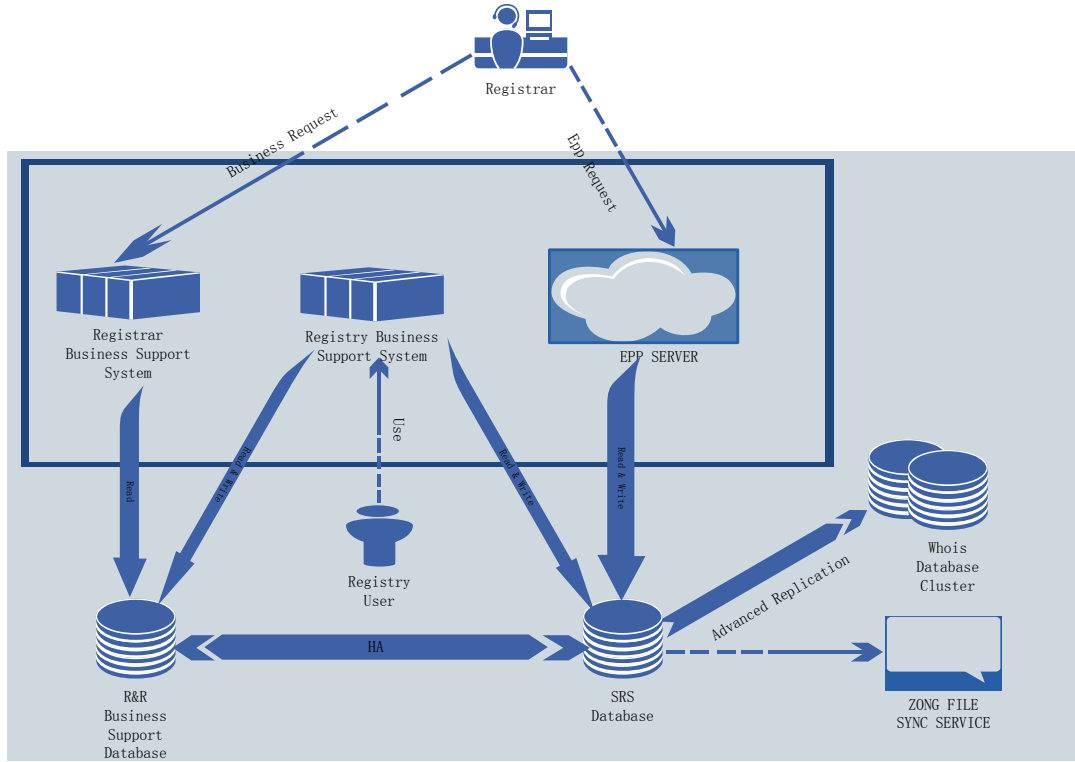
Figure 24-1 System Architecture of SRS
