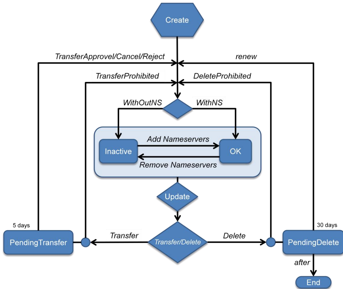
Figure 27-1 Domain Name Lifecycle
