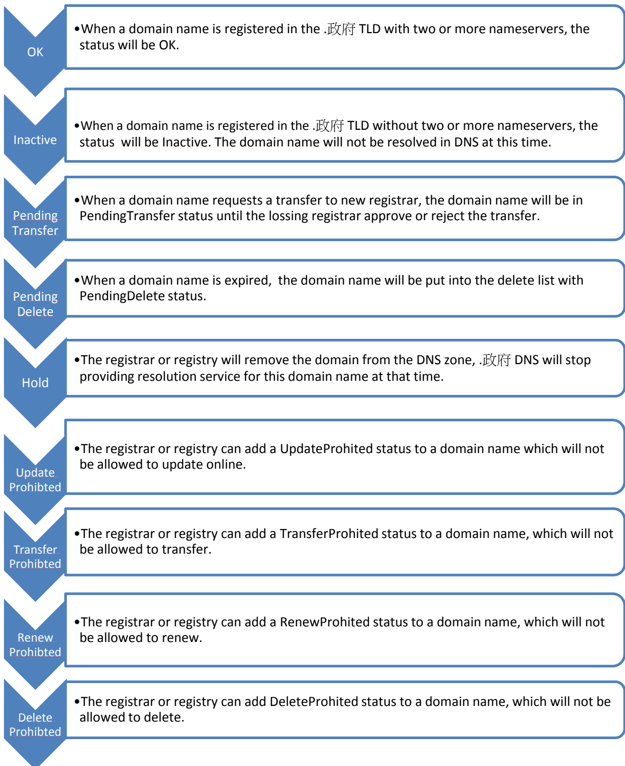
Figure 27-2 Status Description of Domain Name Lifecycle
