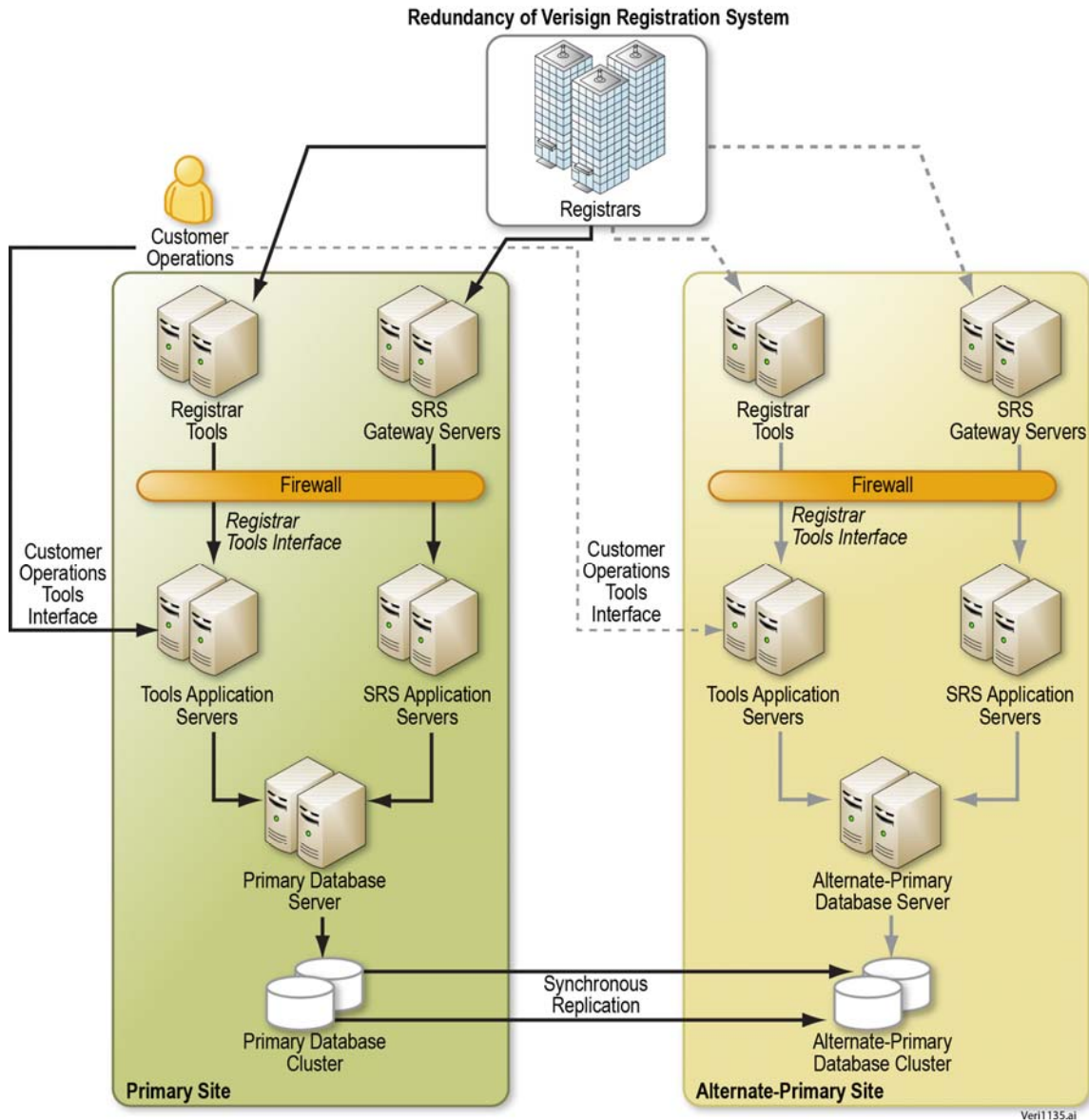
Attachment 24-3: SRS Network Diagram. Verisign’s fully redundant SRS design and geographically separated data centers help ensure service level availability requirements are met.
