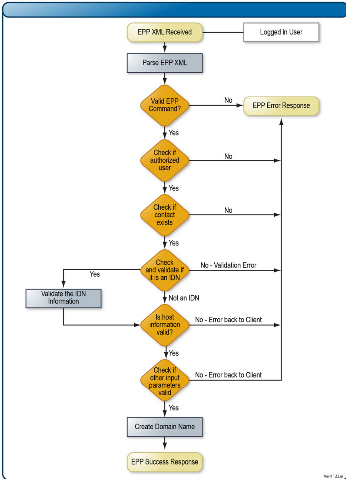
Attachment 27-3: Create Process Flow Chart
