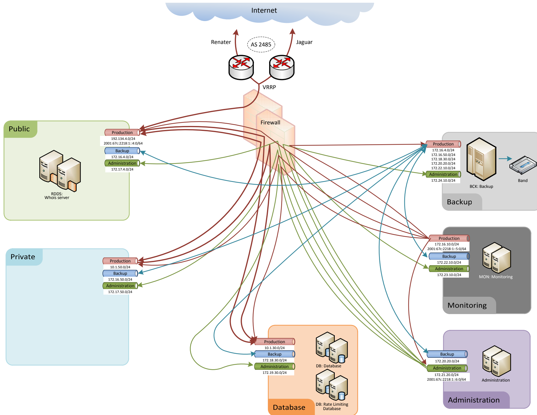
Q26_3 RDSS Architecture Diagram
