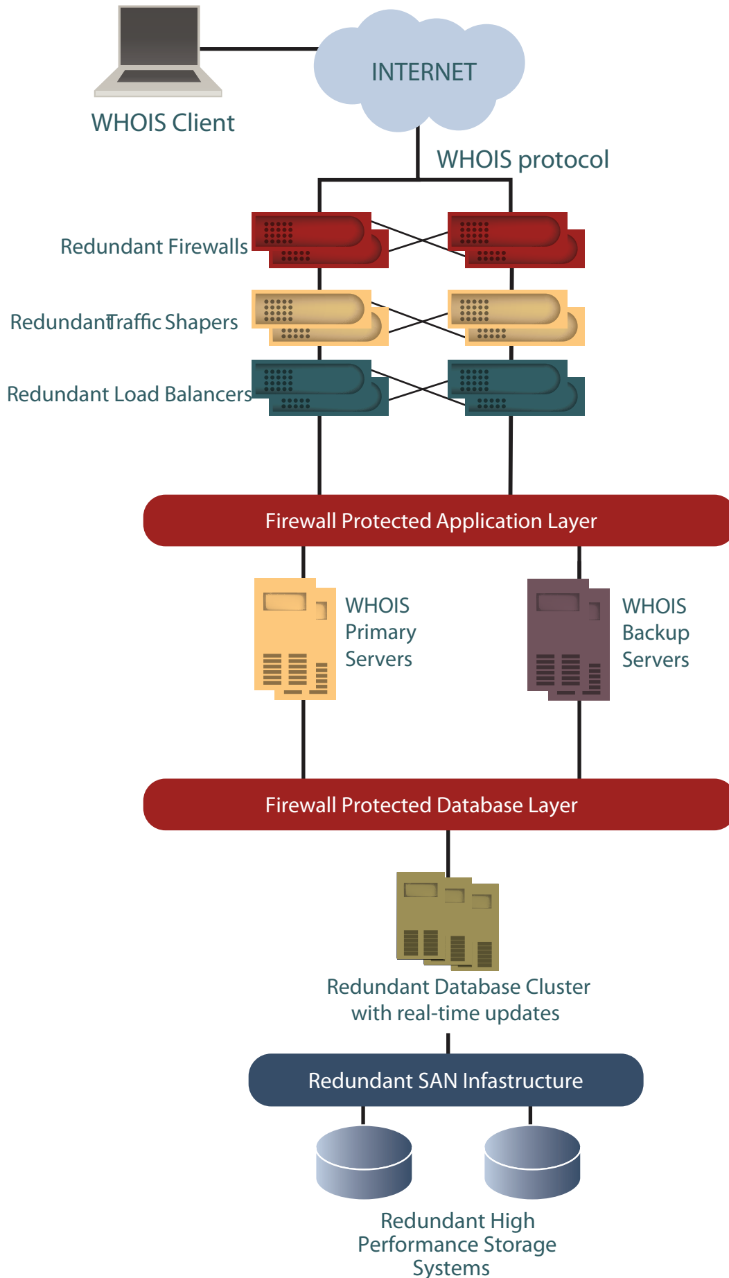
Figure 26-a. WHOIS service diagram.
