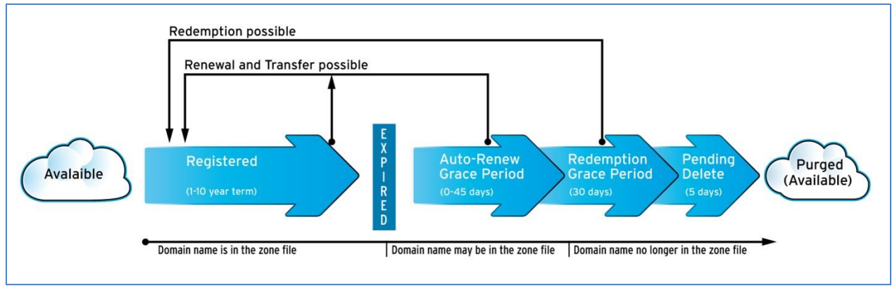
Figure 1: Domain Timeline
