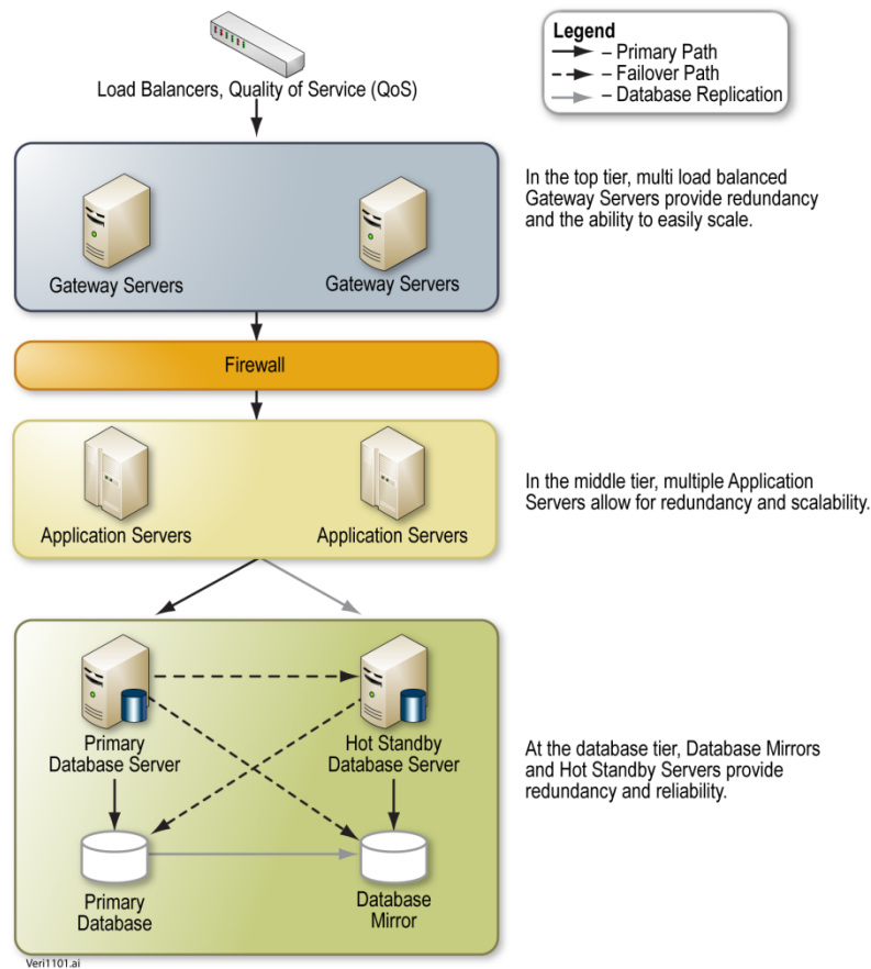
Figure 24-1: SRS Architecture. Verisign's SRS is hierarchically designed to meet the forecasted registration volume of the .SCA gTLD, and it can be scaled to meet future registration volume increases.
