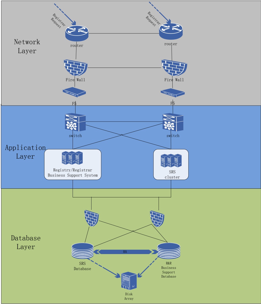
Figure 24-3 Physical Architecture
