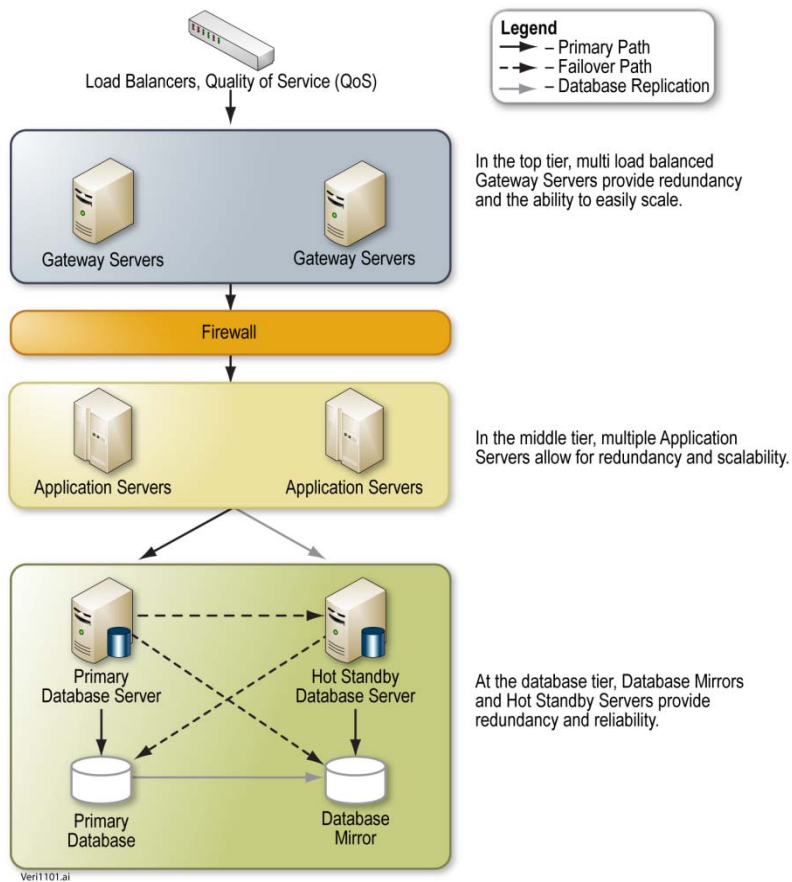
Attachment 24-1: SRS Architecture. Verisign's SRS is hierarchically designed to meet the forecasted registration volume of the .insurance gTLD, and it can be scaled to meet future registration volume increases.
