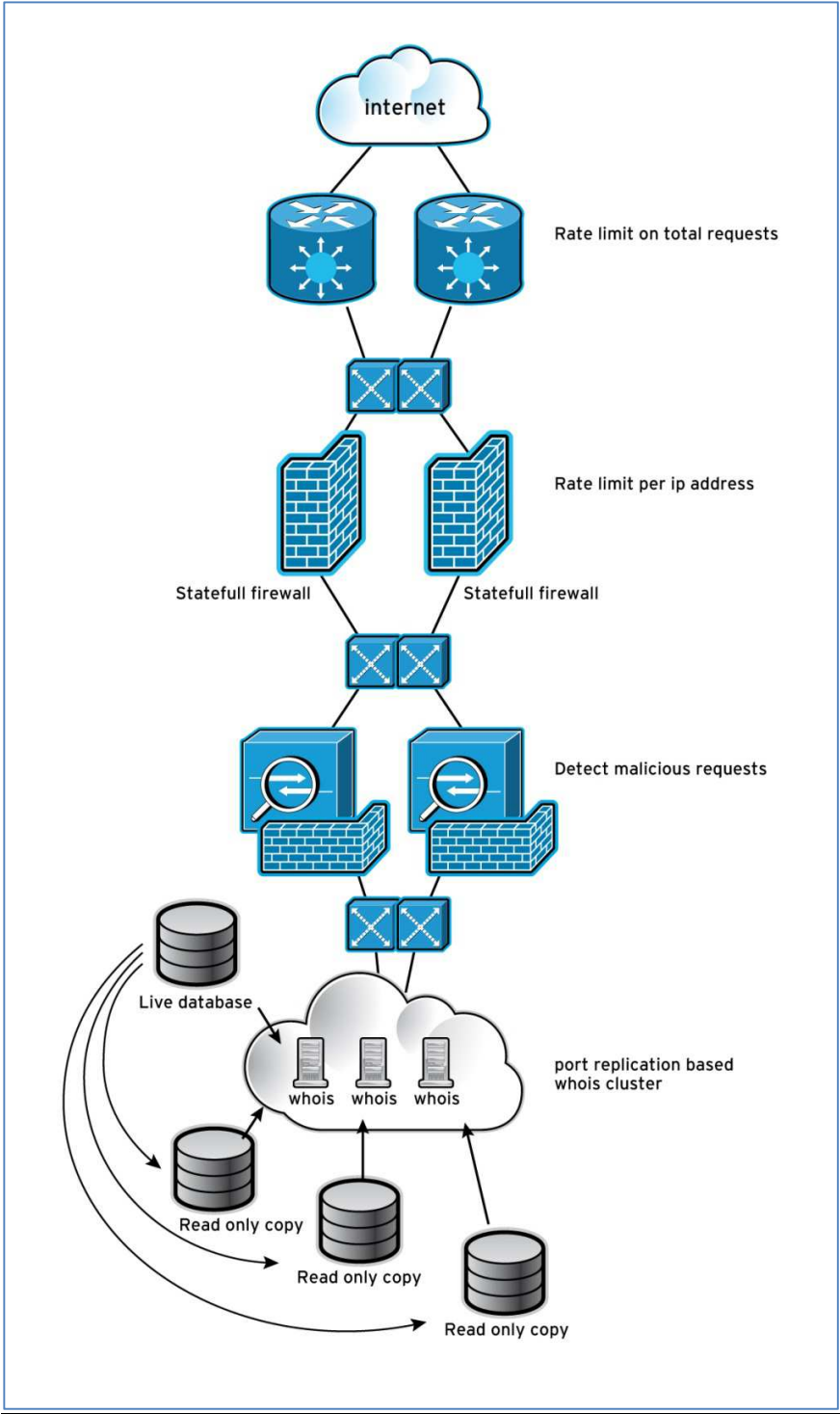
Figure 1: WHOIS Network & Infrastructure Overview
