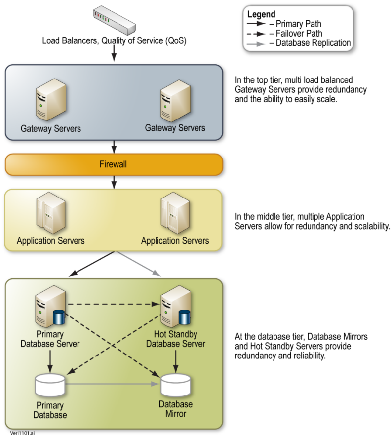
Figure 24-1: SRS Architecture. Verisign's SRS is hierarchically designed to meet the forecasted registration volume of the .webjet gTLD, and it can be scaled to meet future registration volume increases.
