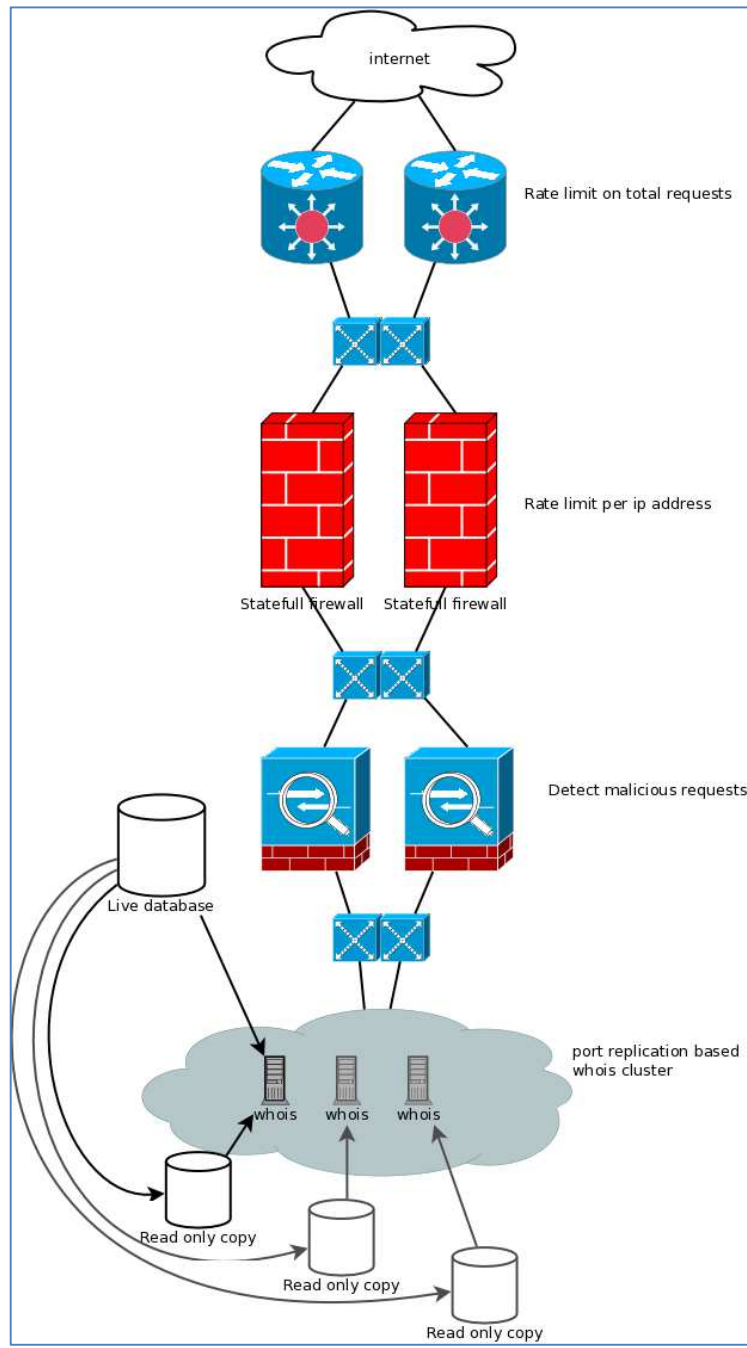
Figure 1: WHOIS Network & Infrastructure Overview
