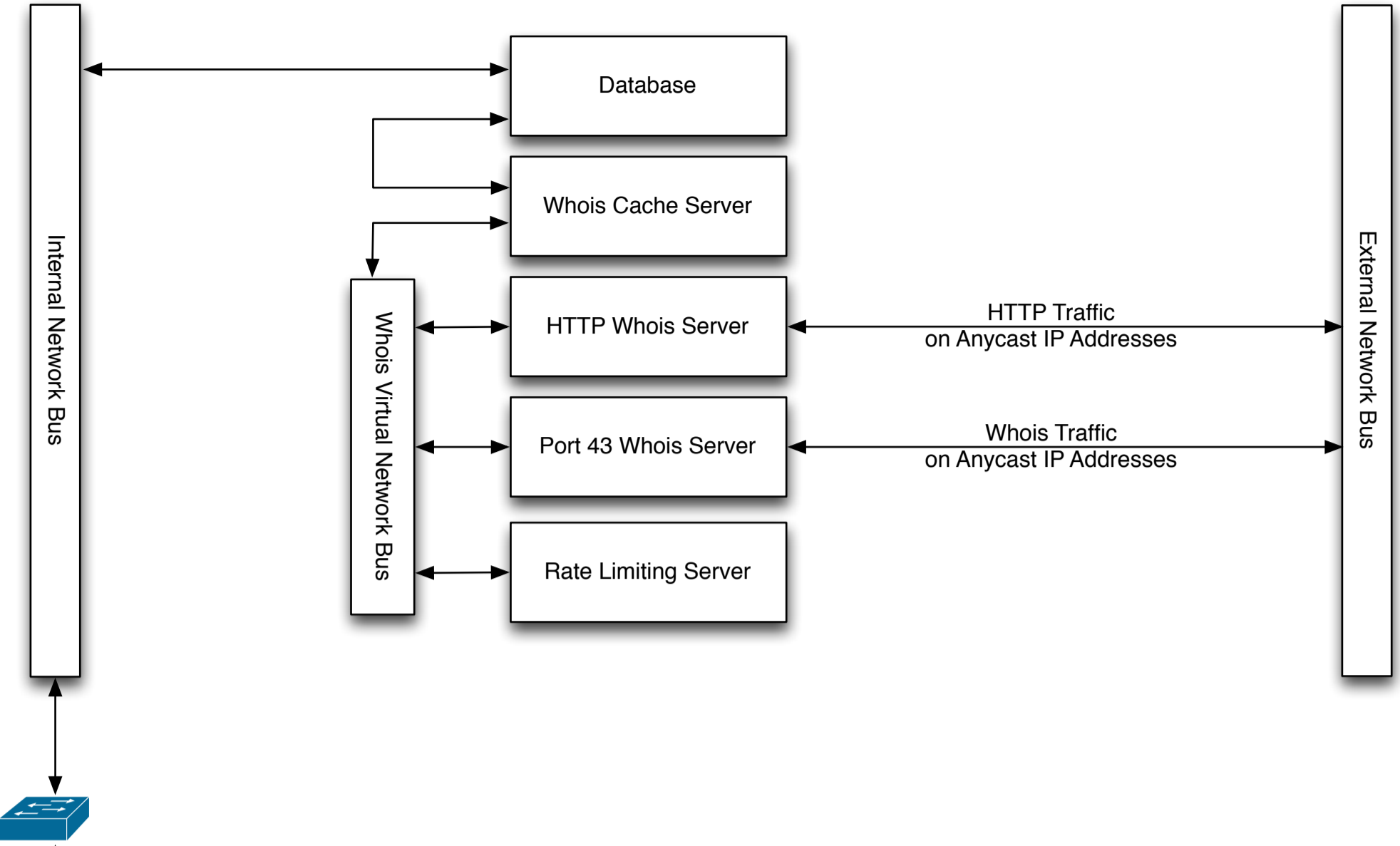
Scalable Master Server Configuration
