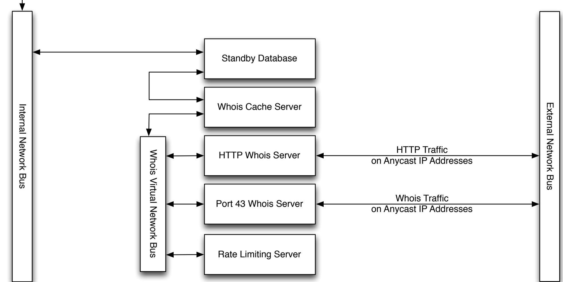
Scalable Remote Standby Server Configuration
