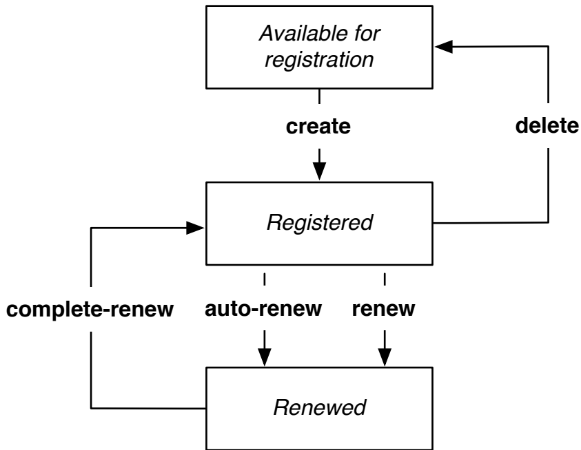
Figure 27.1: registration-renew-cancellation lifecycle
