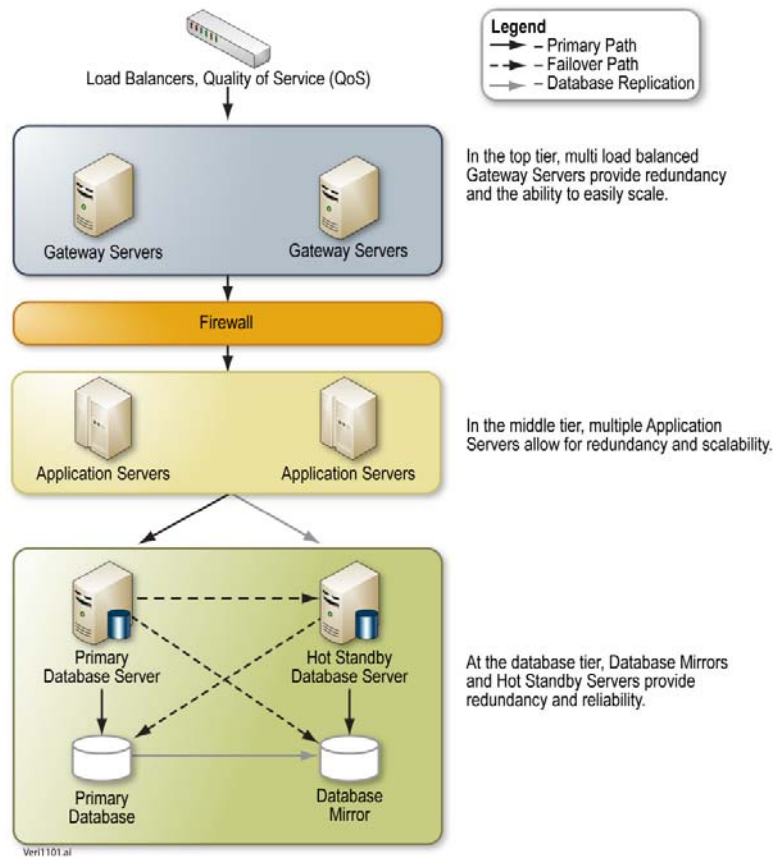
Figure 24-1: SRS Architecture. Verisign's SRS is hierarchically designed to meet the forecasted registration volume of the .nico gTLD, and it can be scaled to meet future registration volume increases.
