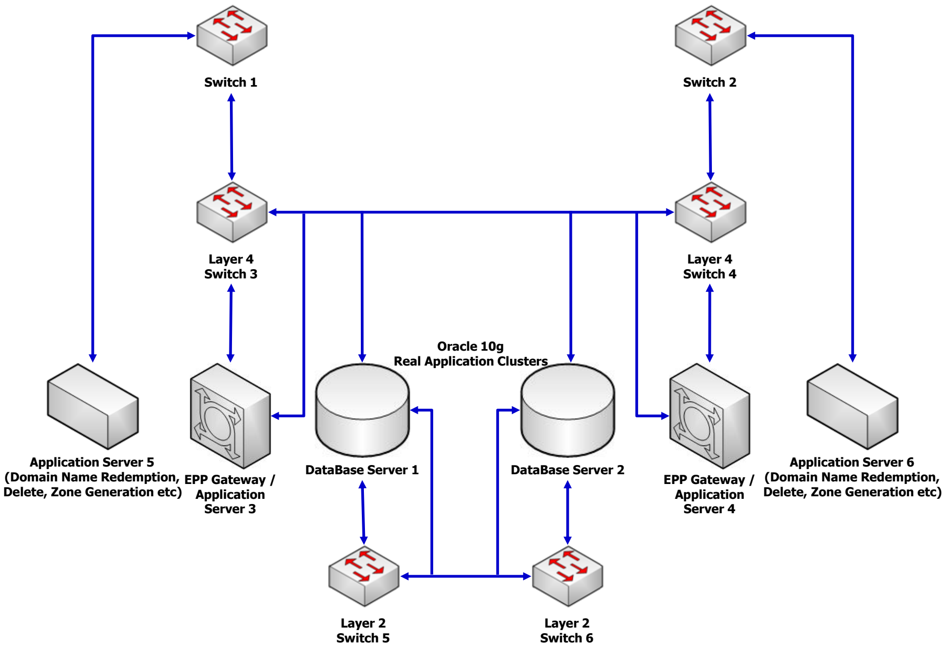
Figure [24-3] SRS Main Center System Architecture
