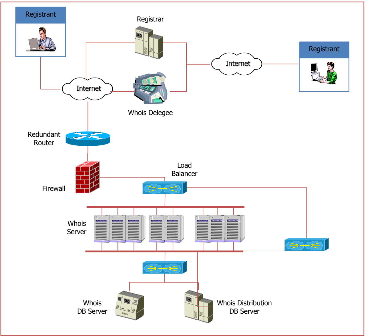
Figure [26-3] Whois Architecture Diagram
