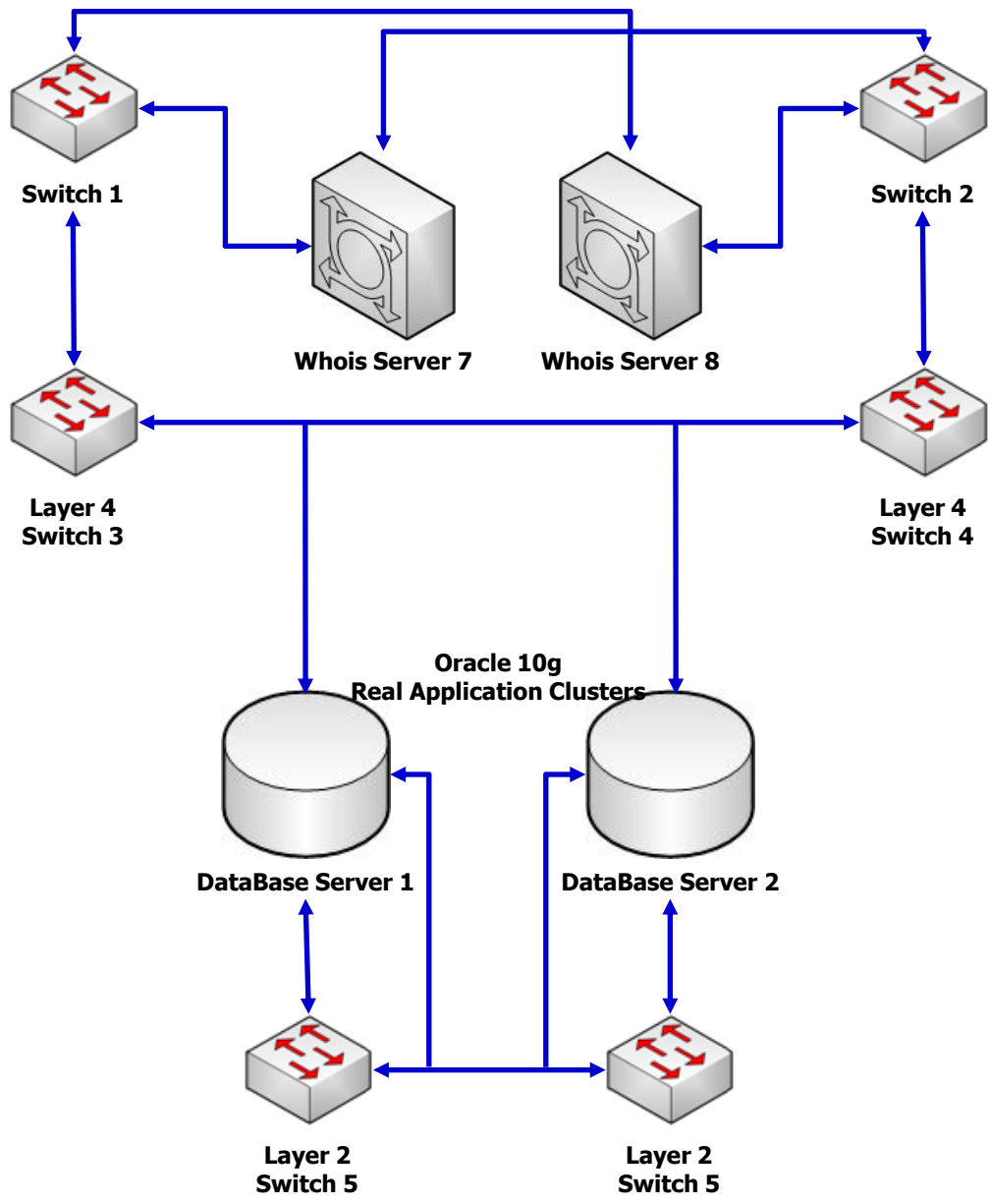
Figure [26-2] Whois System (Main Center)
