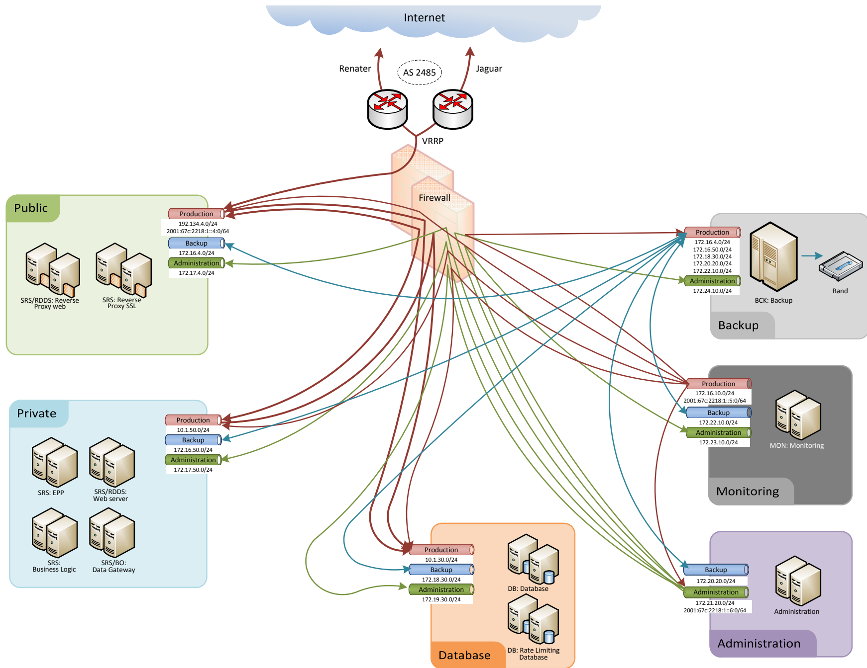
Q24_3 SRS Architecture Diagram
