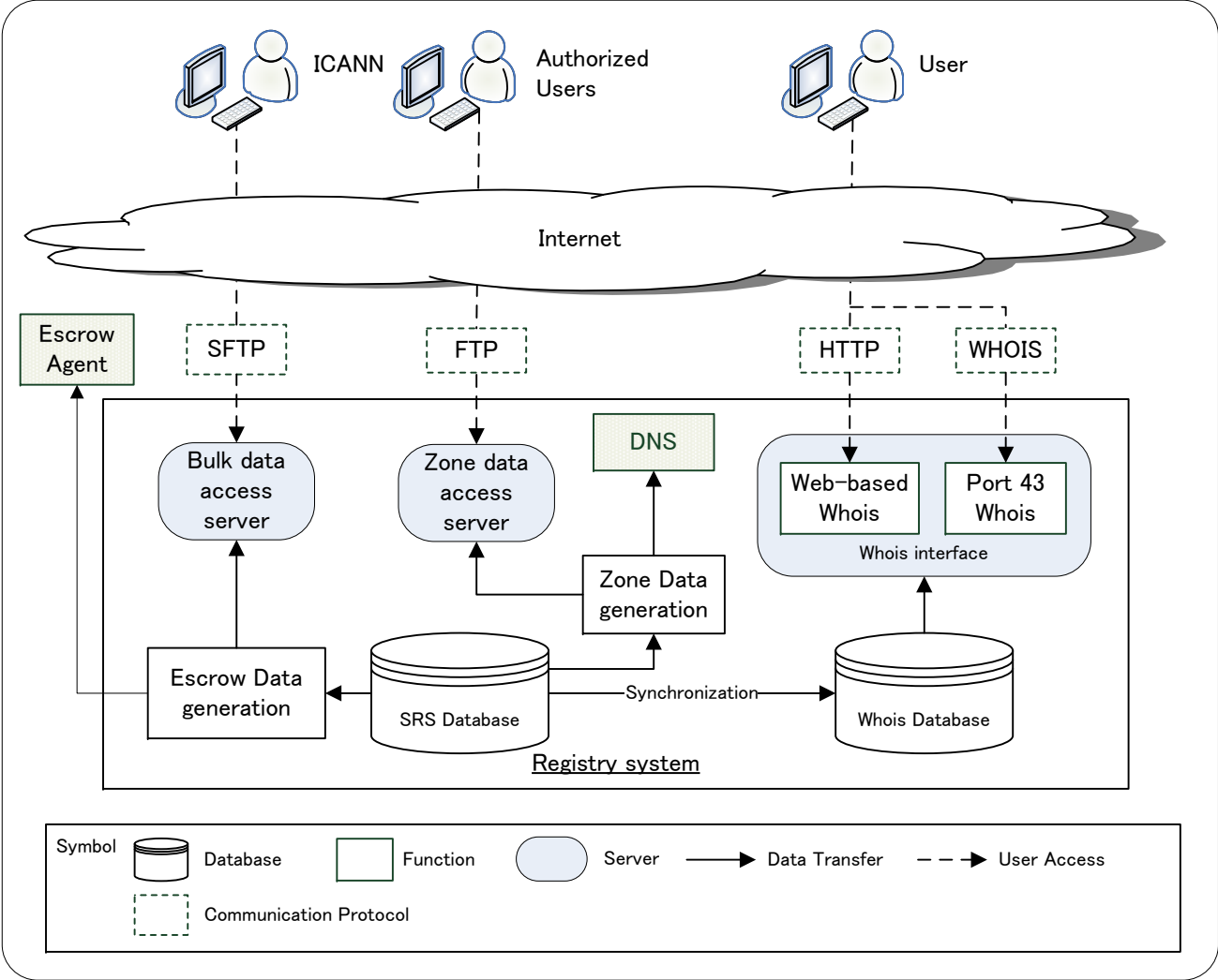
Figure 26-1 Whois System Configuration Diagram
