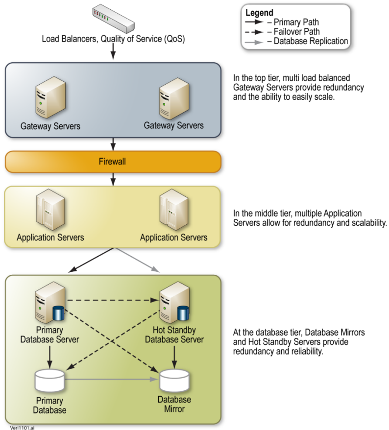
Figure 24-1: SRS Architecture. Verisign's SRS is hierarchically designed to meet the forecasted registration volume of the .broker gTLD, and it can be scaled to meet future registration volume increases.
