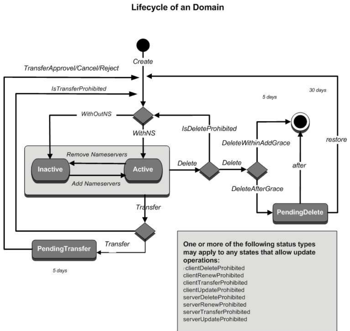
Figure 27-1 Lifecycle of a Domain Name
