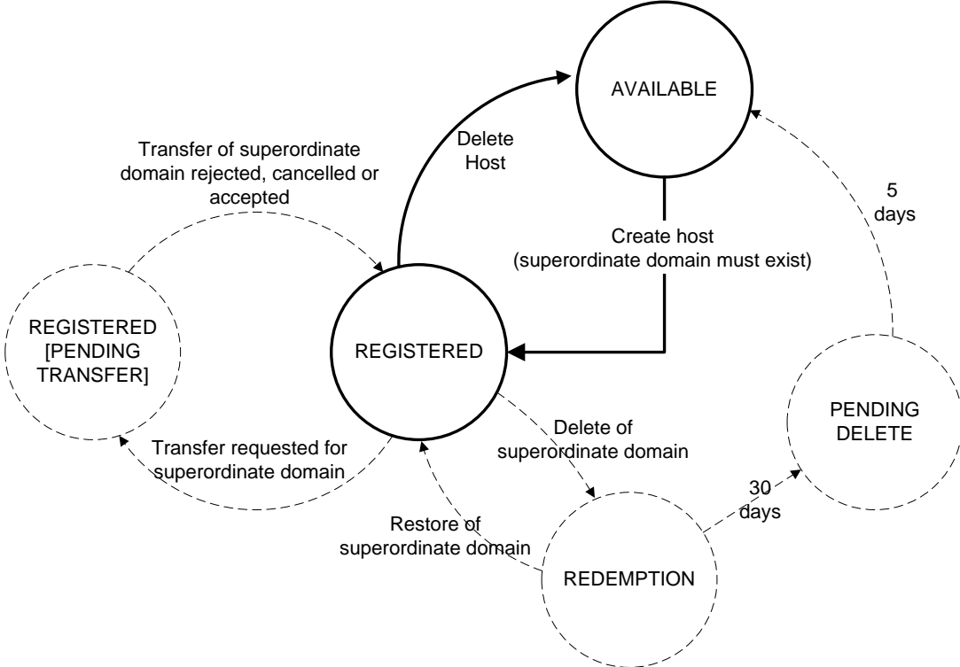
Figure Q27-03: Lifecycle of Internal host objects
