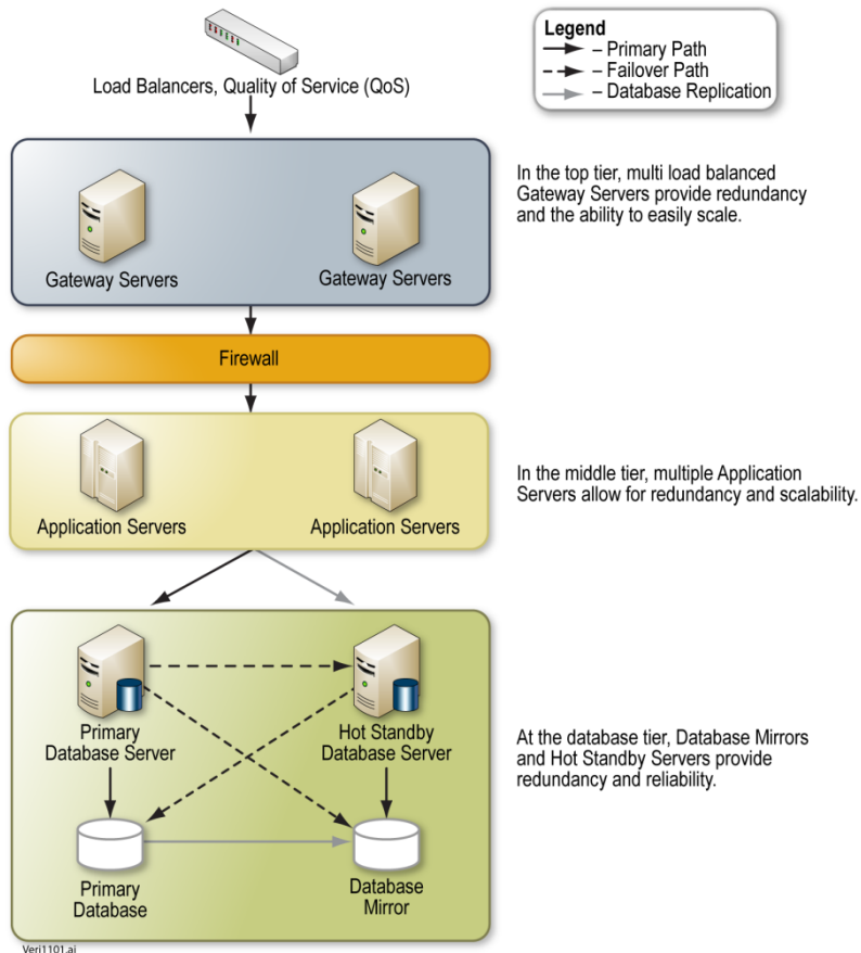
Figure 24-1: SRS Architecture. Verisign's SRS is hierarchically designed to meet the forecasted registration volume of the .ubank gTLD, and it can be scaled to meet future registration volume increases.
