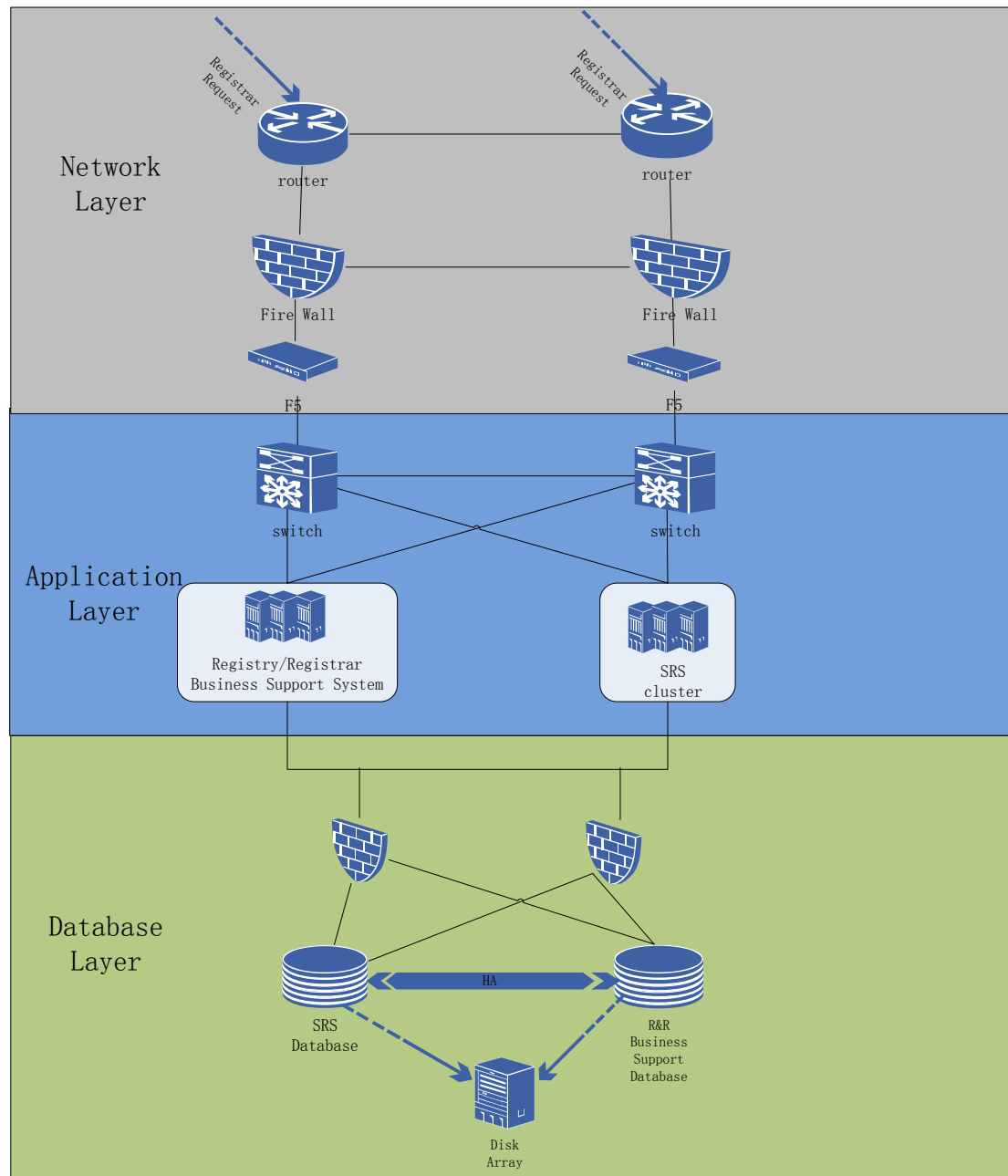
Figure 24-3 Physical Architecture
