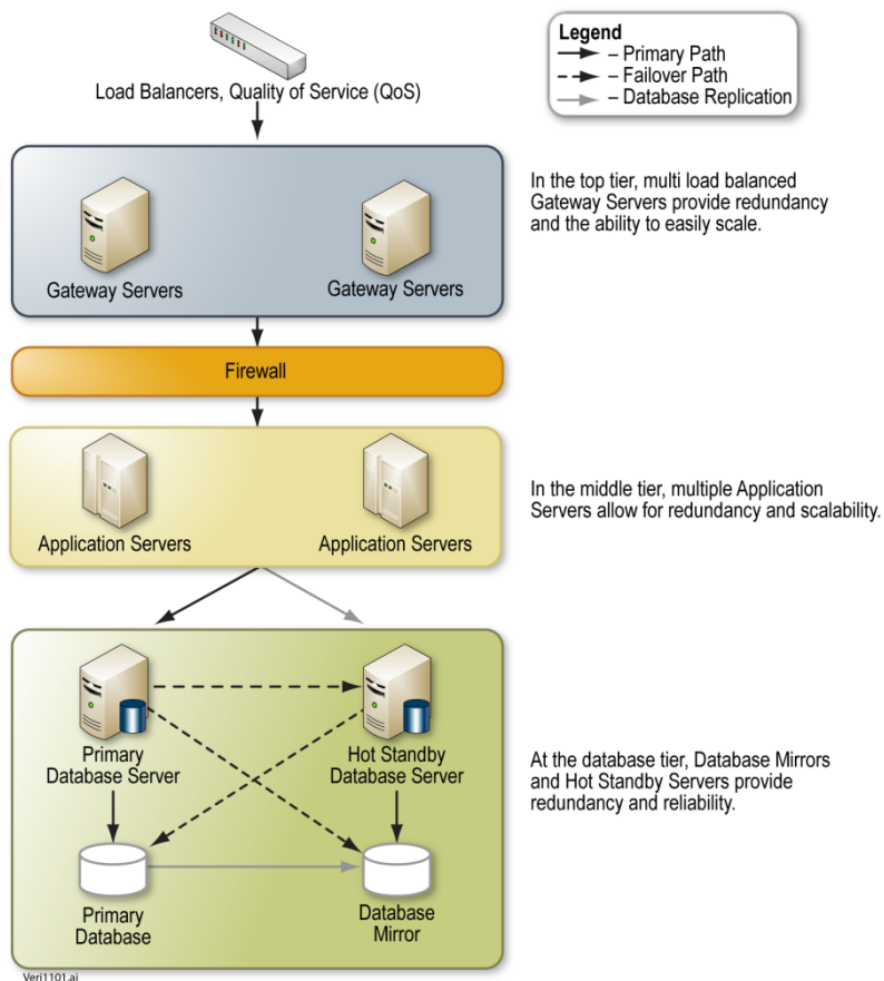
Figure 24-1: SRS Architecture. Verisign's SRS is hierarchically designed to meet the forecasted registration volume of the .ubs gTLD, and it can be scaled to meet future registration volume increases.
